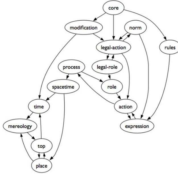
Fig. 1: LKIF modules relations
